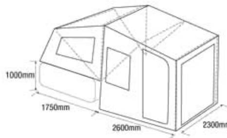
Dimensions for the 7' model
